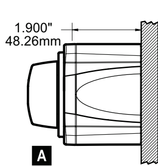
A Surface mounting
