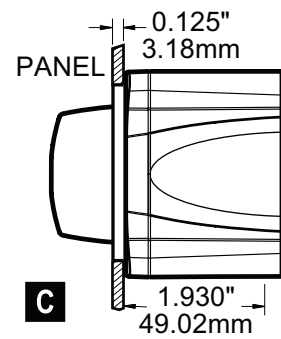
C Rear panel mounting
