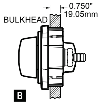
B Front panel mounting
