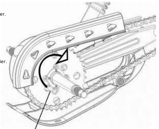
Chain Adjustment Bolt M10X60 Bolt
